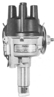
DN-647 Suitable for: Original No. 22100-58002 NISSAN P Engine 6 Cyl
