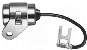
CND-928 MITSUBISHI PART. NO. MD607181 MAZDA PART. NO. 0453-24-322A MITSUBISHI MINICAI MAZDA LUCE, CAPELLA, GRAND FAMILIA, COSMO, 616, 618, 808, R100, COURIER, PICK UP STATION WAGON, SEDAN.
