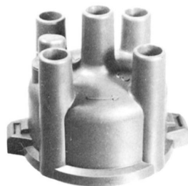
DC-419 TOYOTA PART. NO. 19101-15010 ISUZU PART. NO. 8-94216-730-0 TOYOTA CORSE, TERCEL, AL10(1A-U Eng) ISUZU GEMINI PF50, PF60(G161, G180 Engs) 117COUPE PA95, 96(G180, G2000 Engs)
