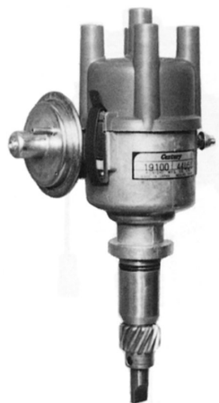
DT-524 Suitable for: Original No. 19100-44030 TOYOTA 5R Engine 4 Cyl
