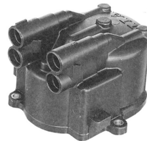
DC-424 TOYOTA PART. NO. 19101-15090 ISUZU PART. NO. 8-94840-106-0
