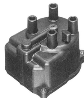
DC-408 HONDA PART. NO. 30102-PM5-A03/A02 PM7-006/016
