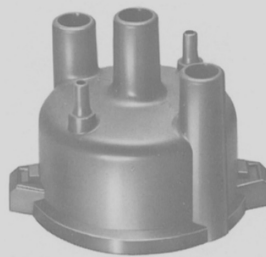
DC-373 DAIHATSU PART. NO. 19101-87702 SUZUKI PART. NO. 33100-74010 DAIHATSU HUET 55, S40, 60, V, VD, VL MAX CUORE L40, L, L45 SUZUKI FRONTE S550, SS11
