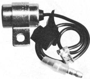
CND-927 MITSUBISHI PART. NO. MD607118 MITSUBISHI GALANT GALANT GTO GALANT Σ LANCER CELESTE,CANTER JEEP
